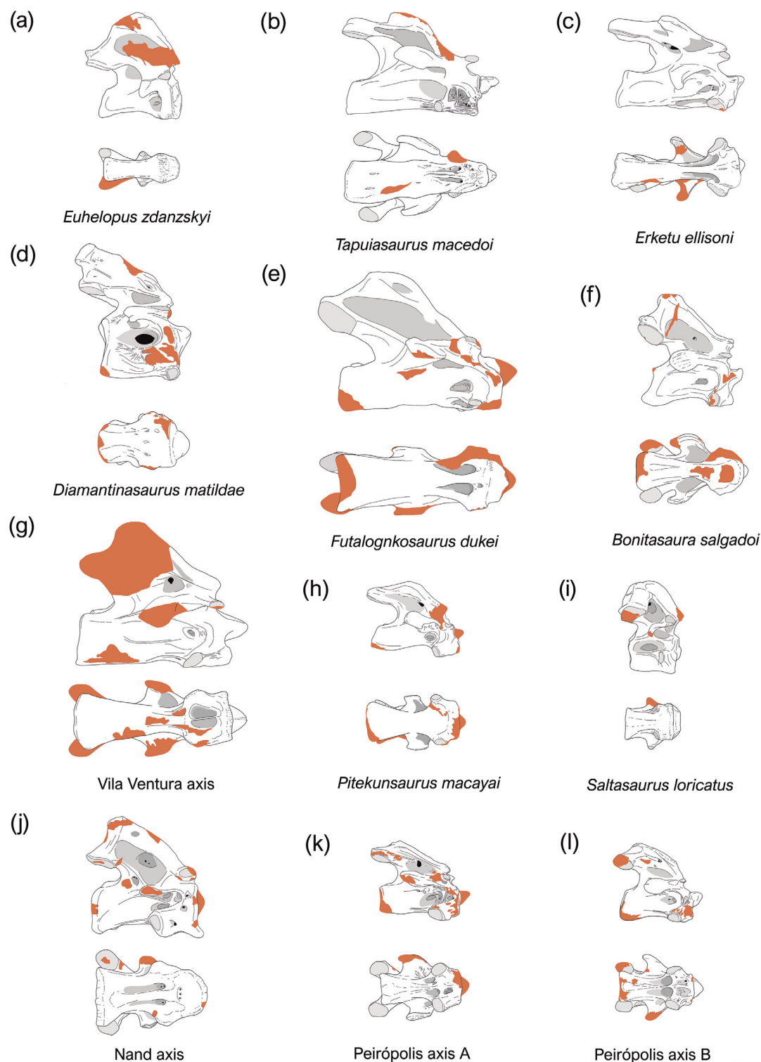
FIGURE 7 Comparisons (to scale) among selected somphospondylan axes in right lateral (top) and ventral (bottom) views: (a) Euhelopus zdanskyi (PMU.R233*); (b) Tapuiasaurus macedoi (MZSP-PV 807*); (c) Erketu ellisoni (IGM 100/1803); (d) Diamantinasaurus matildae (AODF 836*); (e) Futalognkosaurus dukei (MUCPv-323); (f) Bonitasaura salgadoi (MPCA 460*); (g) Vila Ventura axis (MPPC/GPRD 25-013*); (h) Pitekunsaurus macayai (MAU-Pv-AG-446/3); (i) Saltasaurus loricatus (PVL 4017-1); (j) Nand axis (196/CRP/GSI/05); (k) Peirópolis axis A ("DGM Series A", MCT.R.1487); (l) Peirópolis axis B (MCT.R. unnumbered*). Asterisks above indicate reversed views, although reconstructions are based on the most complete structures preserved on either side. Gray tones indicate fossae and articular surfaces, while orange tones represent reconstructed damaged areas. Taxa are ordered in the rows in decreasing order of their geological age. Scale bar equals 5 cm.
