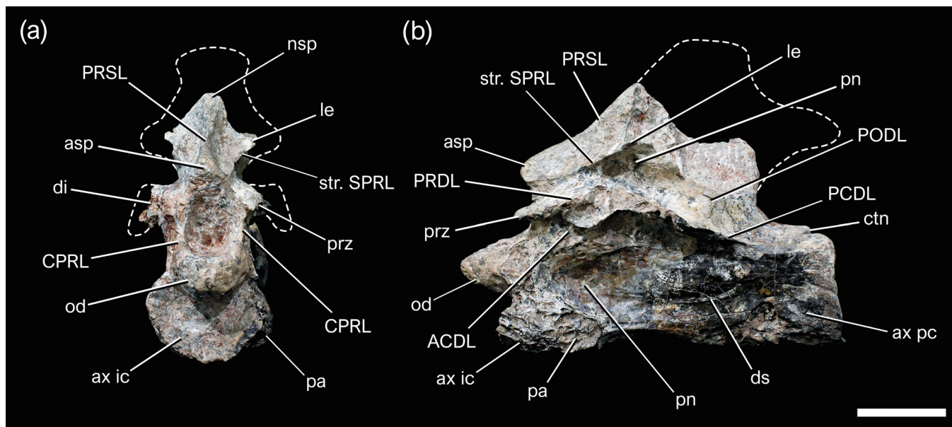
FIGURE 2 The Vila Ventura axis (MPPC/GPRD 25-013) in anterior (a) and left lateral (b) views. Dashed lines represent reconstructed areas, based on the morphology of closely related taxa. Abbreviations: ACDL, anterior centrodiapophyseal lamina; asp, anterior spinal projection; ax ic, axial intercentrum; ax pc, axial pleurocentrum; CPRL, centroprezygapophyseal lamina; ctn, cotylar notch; di, diapophysis; ds, diverticulum scar; le, lateral expansion; nsp, neural spine; od, odontoid; pa, parapophysis; PCDL, posterior centrodiapophyseal lamina; pn, pneumatopore; PODL, postzygodiapophyseal lamina; PRDL, prezygodiapophyseal lamina; PRSL, prespinal lamina; prz, prezygapophysis; str. SPRL, stranded spinoprezygapophyseal lamina. Scale bar equals 5 cm.
